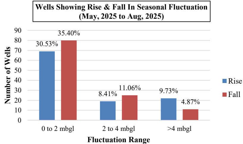
Figure-6: Percentage of wells showing rise and fall in WL in unconfined aquifer (May2025 to Aug 2025)
