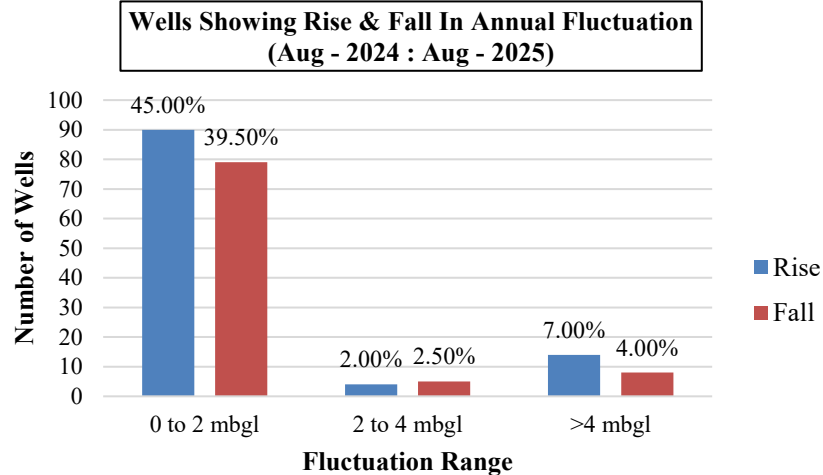
Figure-6: Percentage of wells showing rise and fall in WL in unconfined aquifer (August 2024 to August 2025)
