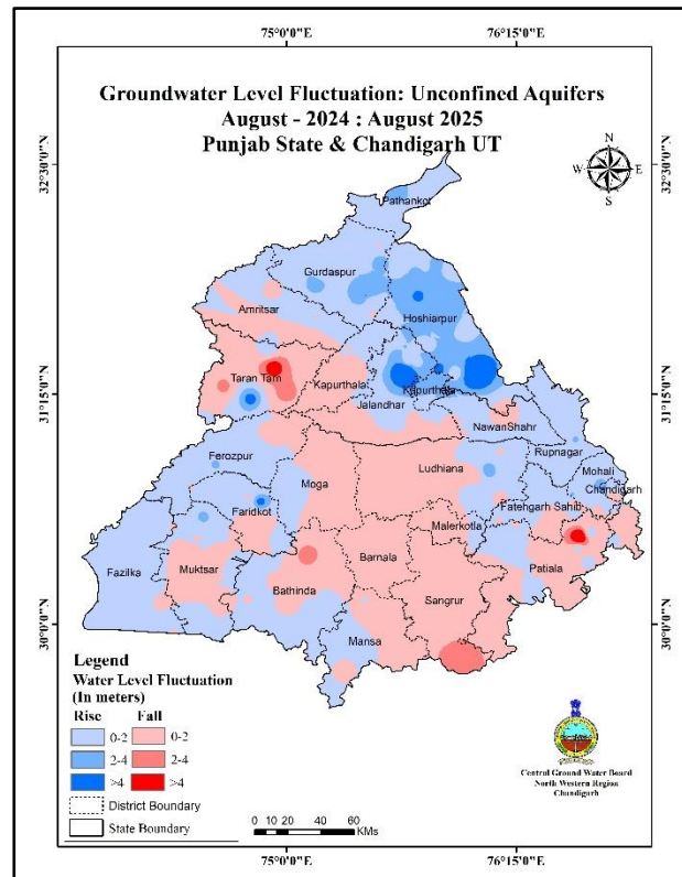
Figure-7: Annual water level fluctuation in unconfined aquifer(August 2024 to August 2025)
