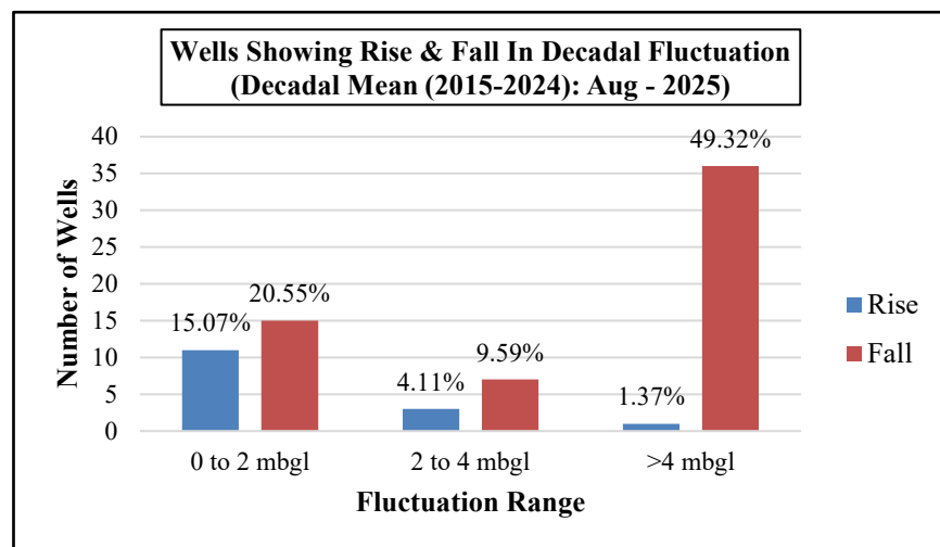
Figure-10: Percentage of wells showing rise and fall in WL in unconfined Aquifer (Decadal Mean Aug (2015-2024) to Aug 2025)
