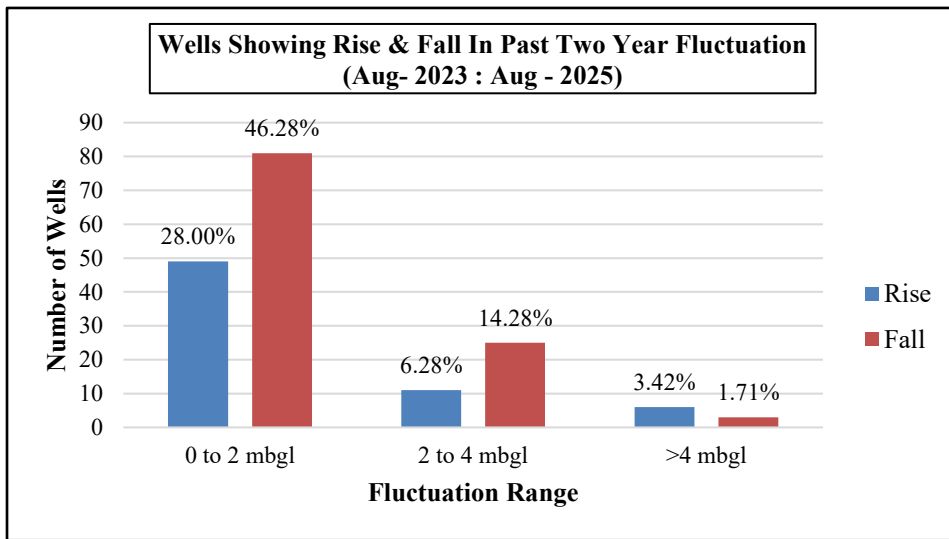
Figure-8: Percentage of wells showing rise and fall in WL in unconfined aquifers (Aug 2023 to Aug 2025)
